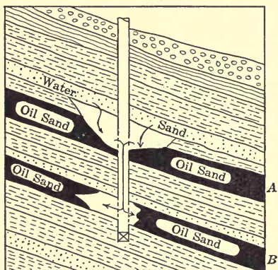
FIG. 72.—Water from top stratum entering zones A and B due to caving of shale above A resulting from withdrawal of sand.
