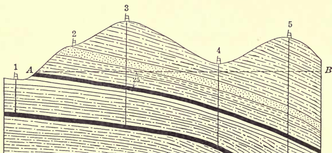
FIG. 37.—Shows effect of topography in choosing well sites.
