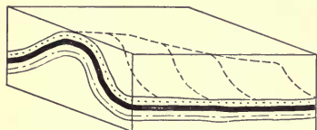
FIG. 35.—Stereogram of plunging anticline.
