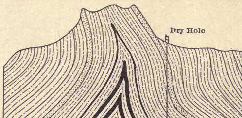
FIG. 10.—Steeply shaped anticline overturned at top.
