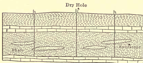
FIG. 16.—Illustrates sand lenses in a shale formation.
