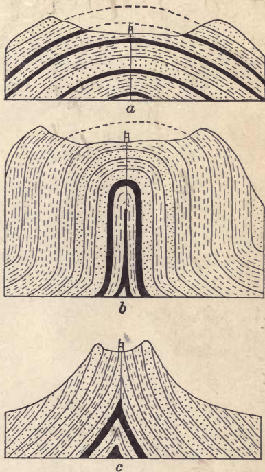
FIG. 8.—Forms of symmetrical anticlines.
