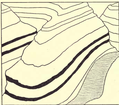
FIG. 39.—Shows how erosion exposes oil sands to drainage.
