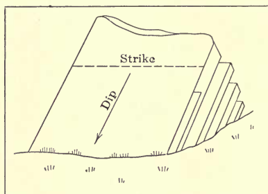
FIG. 36.—Strike and dip. (After Geikie.)
