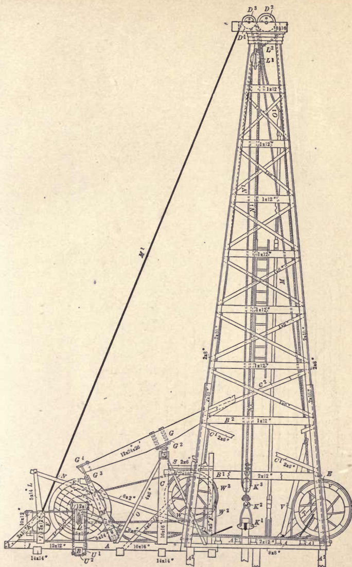
FIG. 52.—Standard cable-tool drilling rig.
